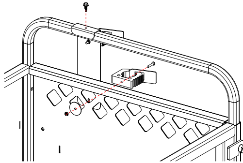
Secures Steel Bracket to Cargo Box
